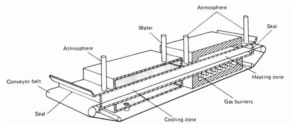
Continuous conveyor furnace for heat treating copper alloys in a controlled atmosphere. Source: ASM Handbook, Vol. 4, Heat Treating , ASM International, 1991, p 887
