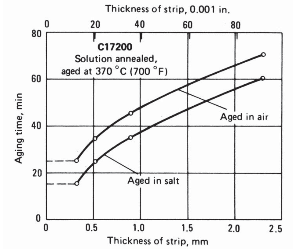
Effect of metal thickness and heating medium on aging time required to develop maximum strength in C17200 (wrought beryllium-copper) strip. Source: ASM Handbook, Vol. 4, Heat Treating , ASM International, 1991, p 888
