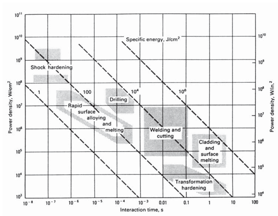
Interaction times and power densities necessary for various laser surface modification processes. Source: J.R. Davis, Ed., Cast Irons , ASM Specialty Handbook, ASM International, 1996, p 188
