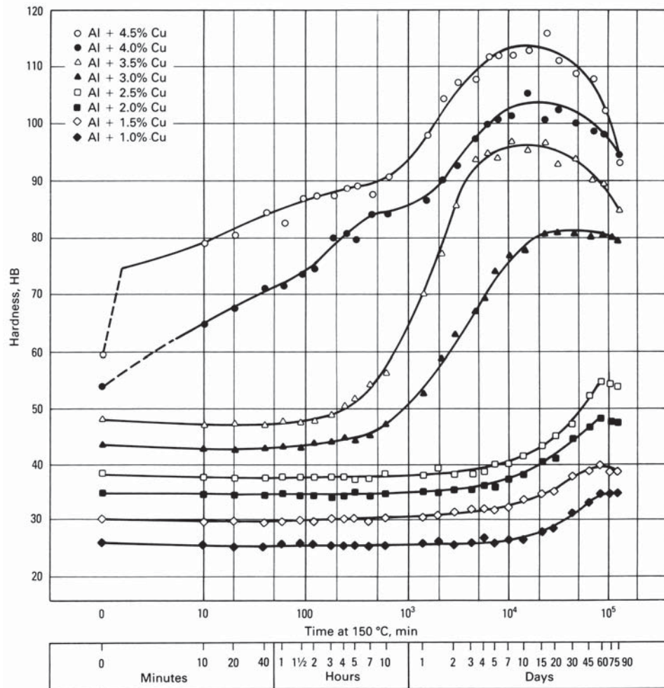
Precipitation hardening curves for binary Al-Cu alloys quenched in water at 100°C (212°F) and aged at 150°C (300°F). Source: J.R. Davis, Ed., Aluminum and Aluminum Alloys , ASM Specialty Handbook, ASM International, 1993, p 36
