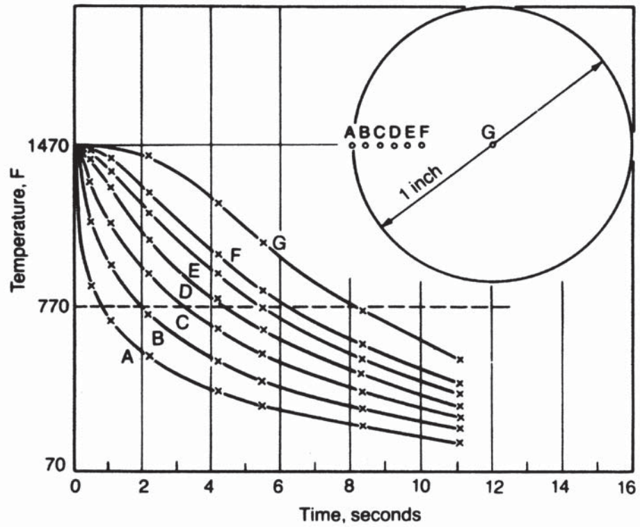
Cooling curves at various positions in a 1 in. (25.4 mm) diameter bar quenched with a severity of quench H = 4 . Source: Steels: Processing, Structure, and Performance , George Krauss, Fifth Edition, ASM International, 2005, p 308
