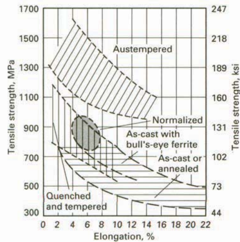
Tensile strength versus elongation of ductile iron; (top) minimum values of austempered ductile iron grades specified in ASTM A897; (bottom) range of tensile strength and elongation values with different heat treatments. Source: J.R. Davis, Ed., Cast Irons , ASM Specialty Handbook, ASM International, 1996, p 194
