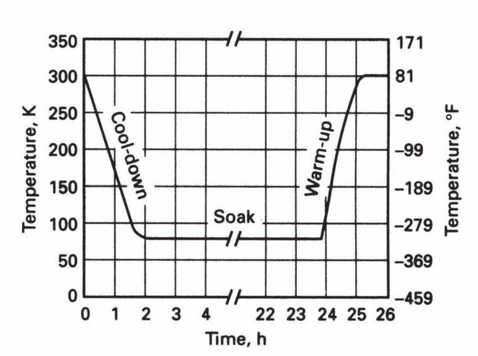
Plot of temperature versus time for the cryogenic treatment process. Source: ASM Handbook, Vol. 4, Heat Treating , ASM International, 1991, p 204
