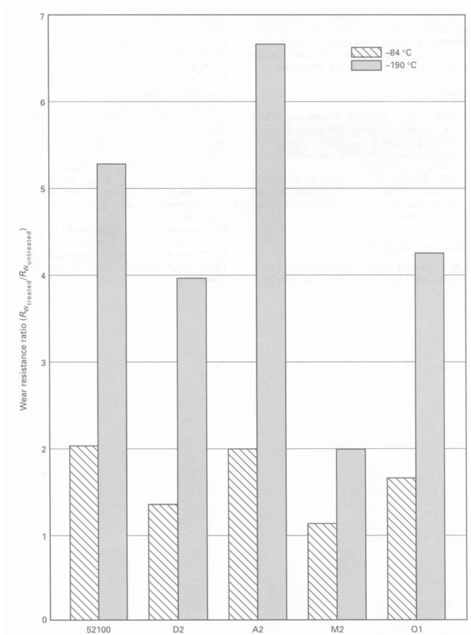
Comparison of wear-resistance ratios for five high-carbon steels soaked at -84 and -190°C (-120 and -310°F). Soaking temperatures below -84°C does not significantly change the hardness of the material. Source: ASM Handbook, Vol. 4, Heat Treating , ASM International, 1991, p 205
